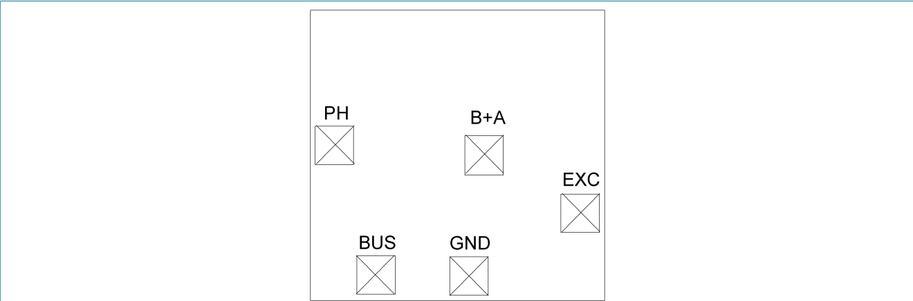
Figure 4. AR6000 pinout diagram
