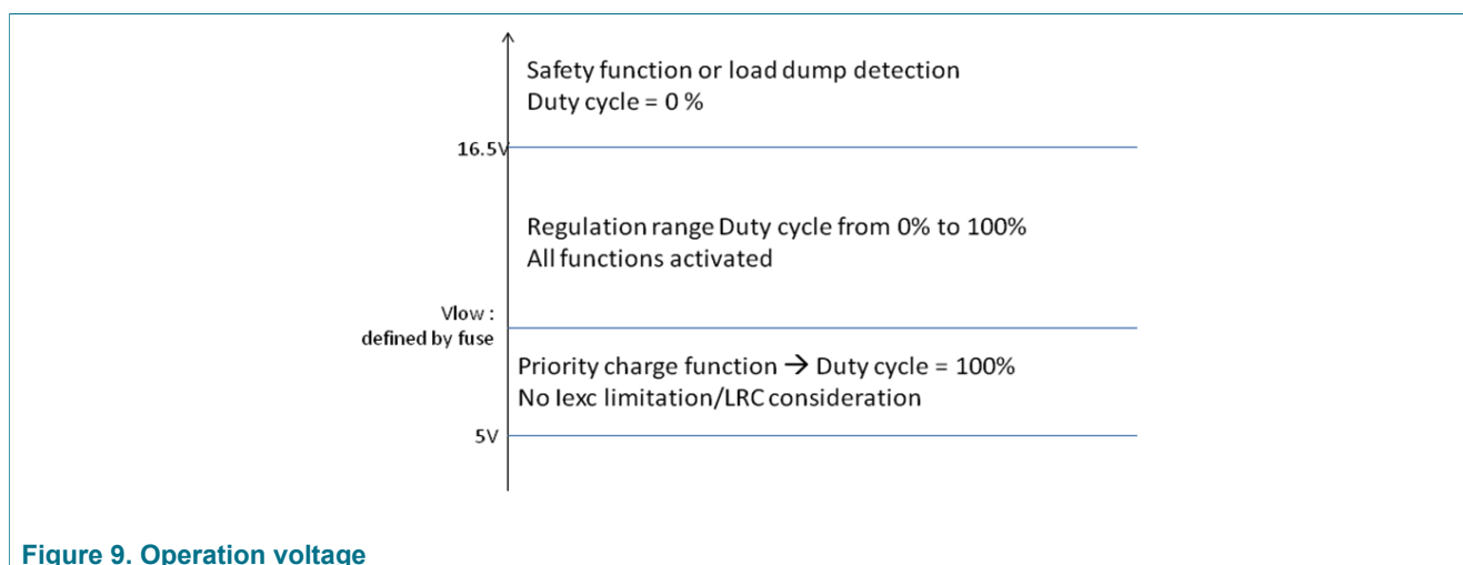
Figure 9. Operation voltage
