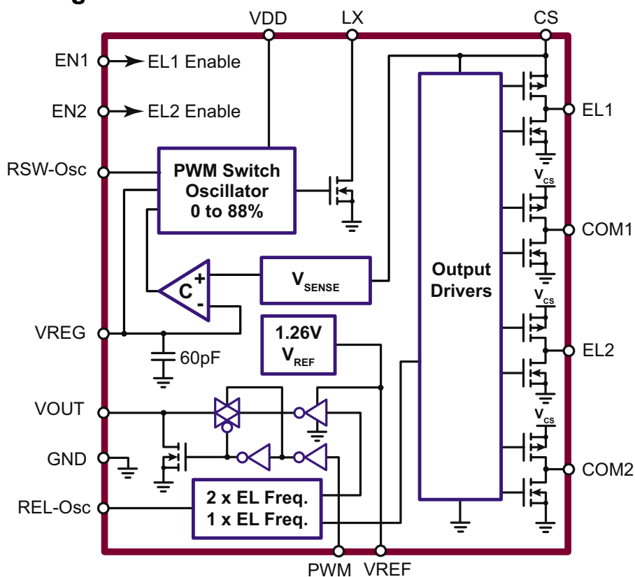
Figure 1: Block Diagram
