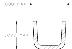
SECTION D-D SCALE 20:1
