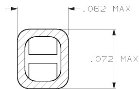
SECTION E-E SCALE 20:1
