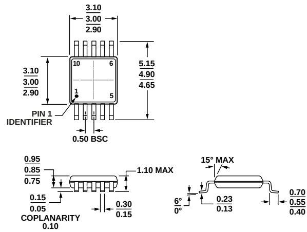
Figure 11. 10-Lead Mini Small Outline Package [MSOP] (RM-10)
