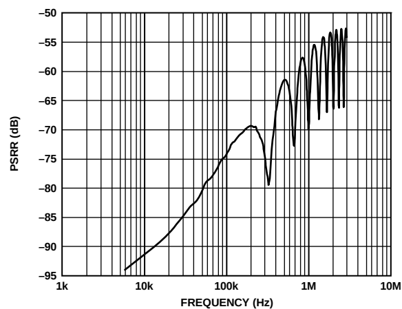
Figure 33. I_{SENSE} Power Supply Rejection Ratio vs. Supply Ripple Frequency Without V_{PP} Supply Decoupling Capacitors for a 500 mV Ripple
