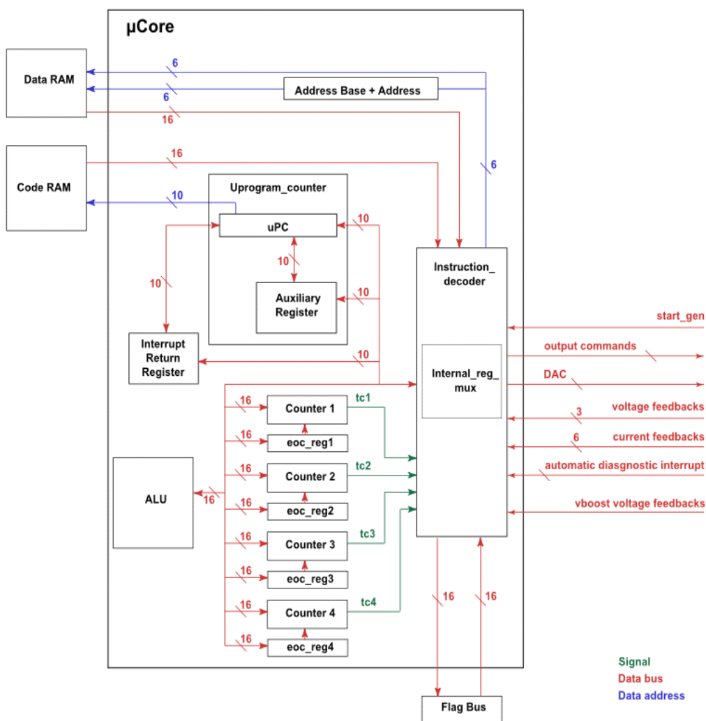
Figure 34. Microcore block diagram
