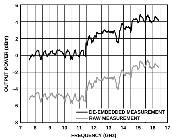
Figure 17. RF16P and RF16N Output Power, De-Embedded Board and Cable Measurement, Combined Using Balun
