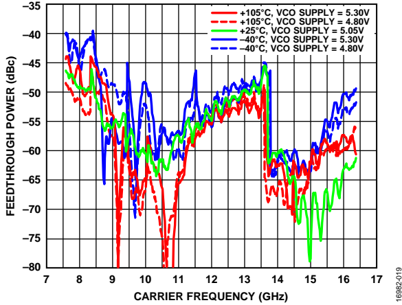
Figure 19. RF16P and RF16N VCO × 3 Feedthrough, De-Embedded Board and Cable Measurement, Combined Using Balun
