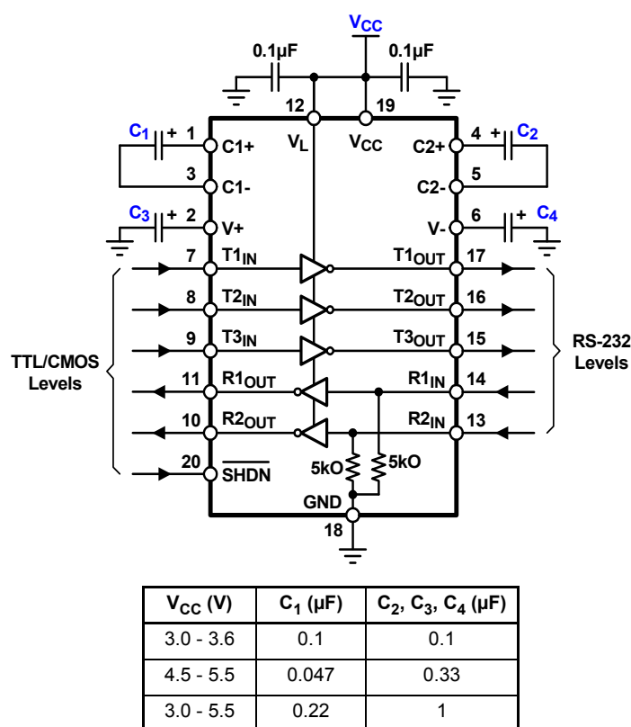
Figure 1. Typical Operating Circuit
