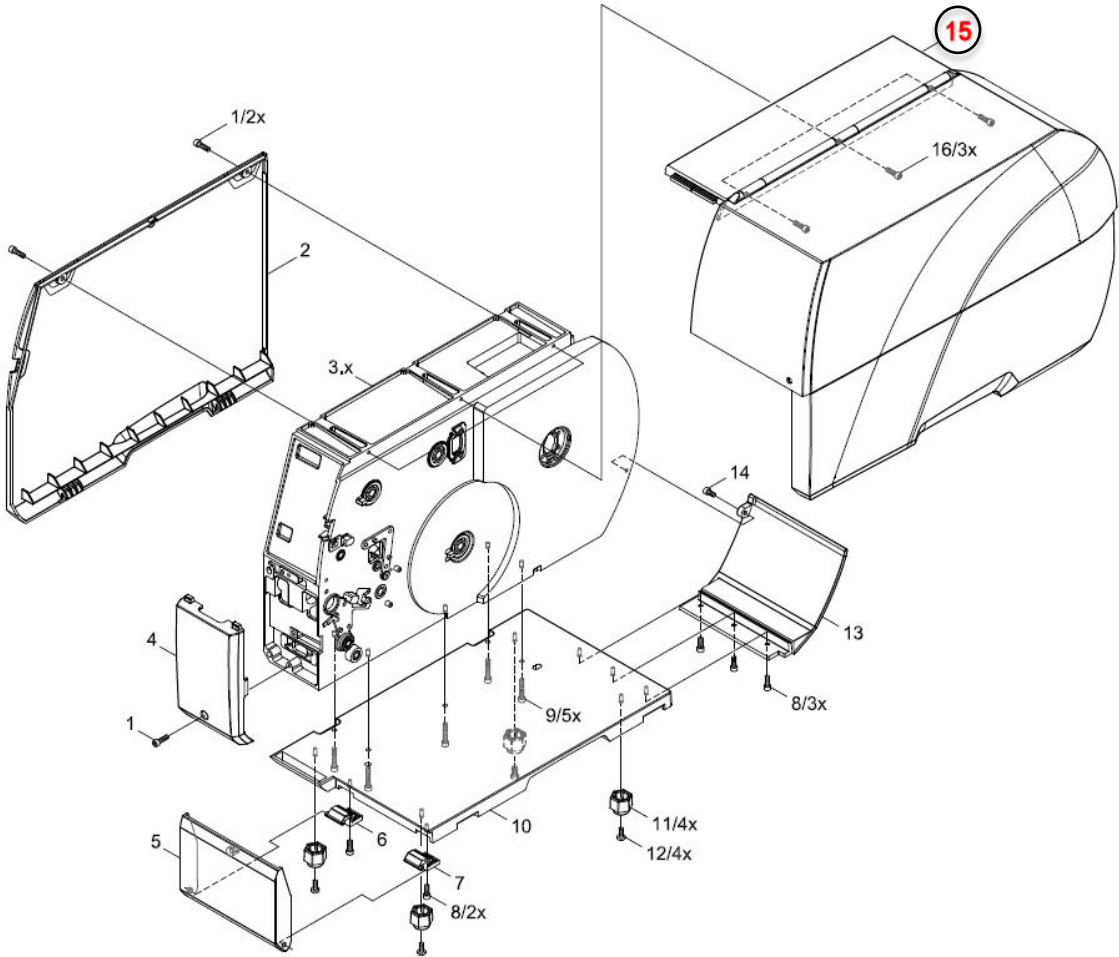
Figure 3 – T3212/T3224-PRINTER (cover)
