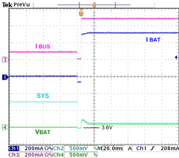
Figure 19. Charger Enable ( CE\# = 1-0 ) with V_{BUS} Applied, I_{BUSLIM}=500\text{ mA} , 200\text{ mA SYS Load} , IO\_LVL=0
