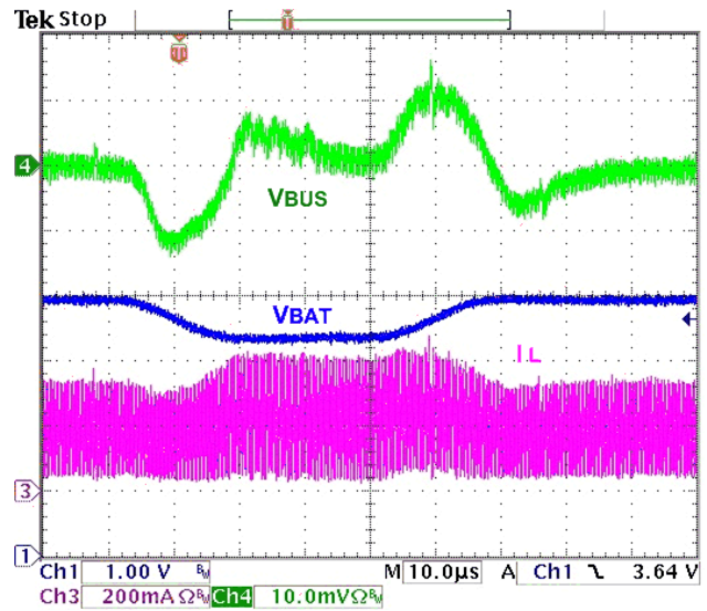
Figure 32. Line Transient, 50 Ω Load, 3.9-3.3- 3.9 V BAT , t_{RISE/FALL}=10\text{ µs}
