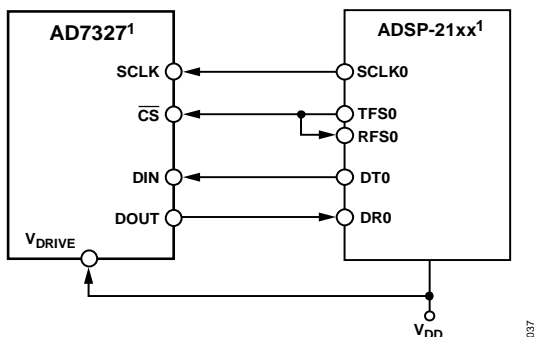
Figure 54. Interfacing the AD7327 to the ADSP-21xx
