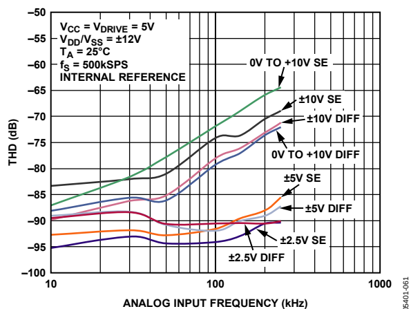
Figure 11. THD vs. Analog Input Frequency for Single-Ended (SE) and True Differential Mode (Diff) at 5 V V_{CC}
