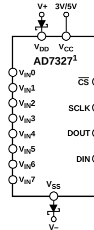
Figure 56. Schottky Diode Connection
