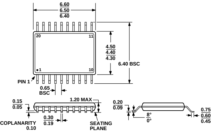
COMPLIANT TO JEDEC STANDARDS MO-153-AC Figure 57. 20-Lead Thin Shrink Small Outline Package [TSSOP] (RU-20) Dimensions show in millimeters
