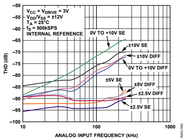
Figure 10. THD vs. Analog Input Frequency for Single-Ended (SE) and True Differential Mode (Diff) at 3 V V_{CC}
