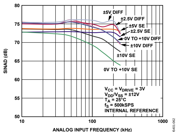
Figure 12. SINAD vs. Analog Input Frequency for Single-Ended (SE) and True Differential Mode (Diff) at 3 V V_{CC}
