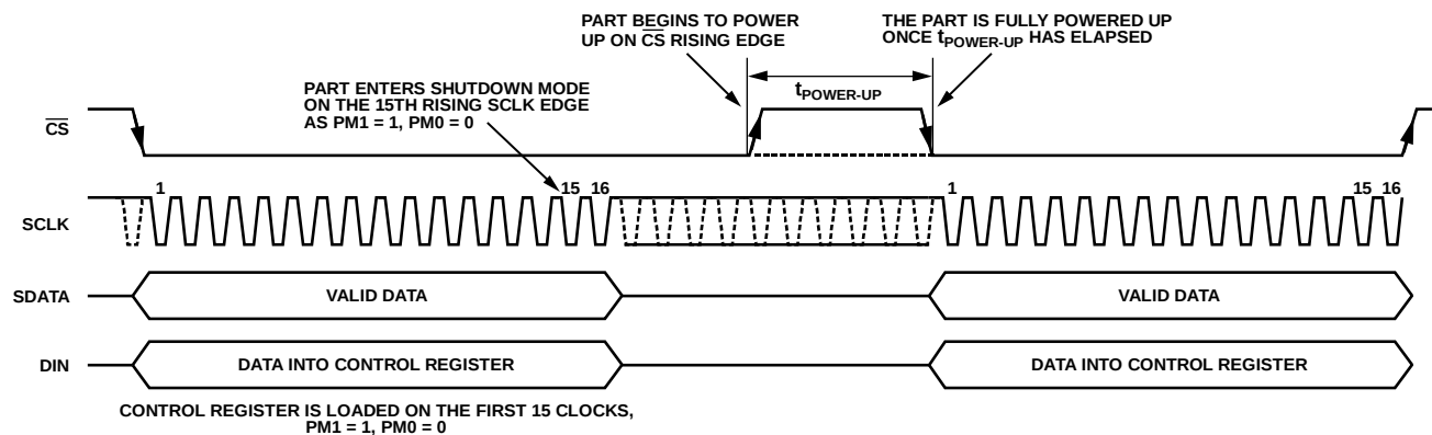
Figure 50. Entering Autoshtutdown/Autostandby Mode
