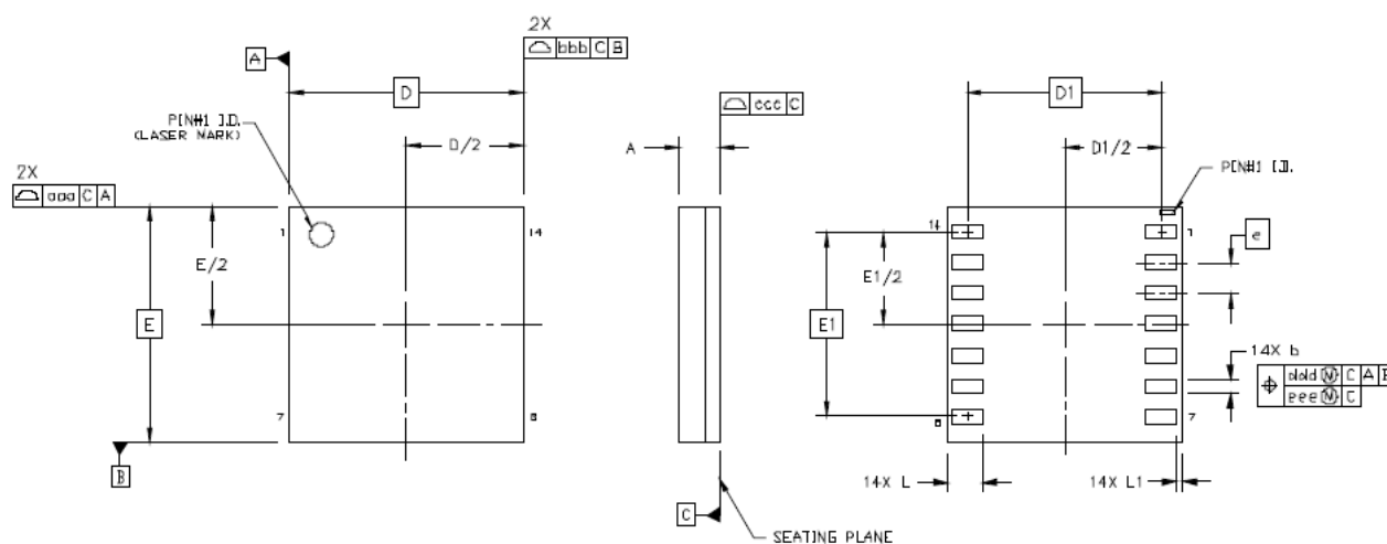
Figure 6.4. Si823x LGA Outline
