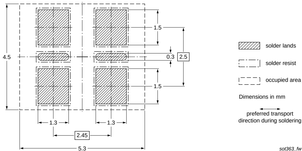
Fig 20. Wave soldering footprint PUMD15 (SOT363)
