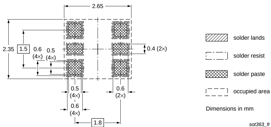
Fig 19. Reflow soldering footprint PUMD15 (SOT363)
