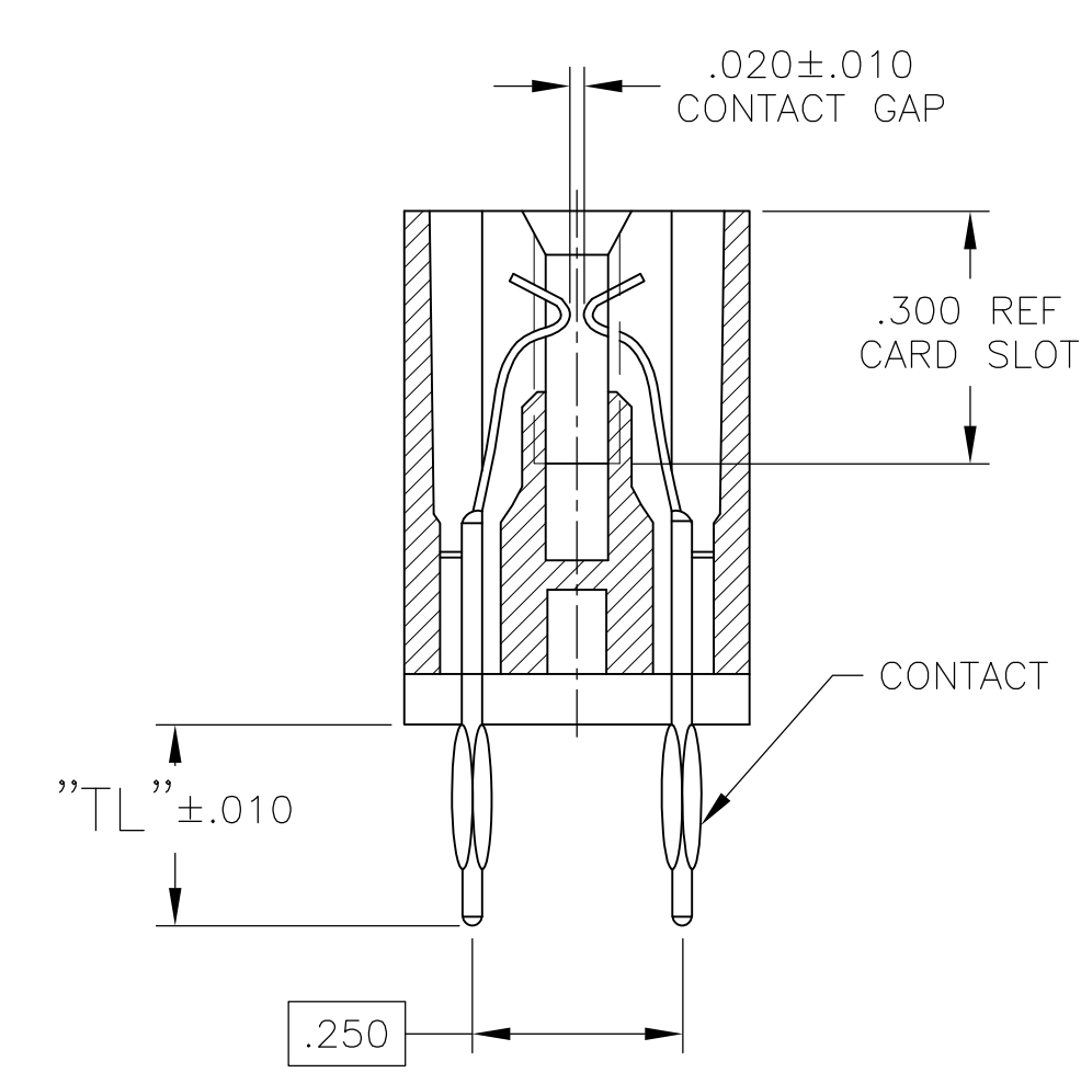
SECTION E-E
