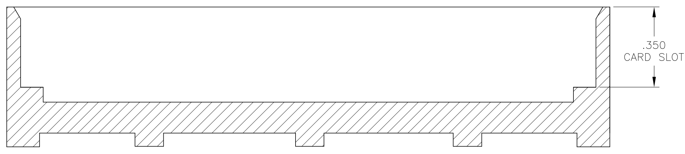
MOUNTING STYLE "13"
