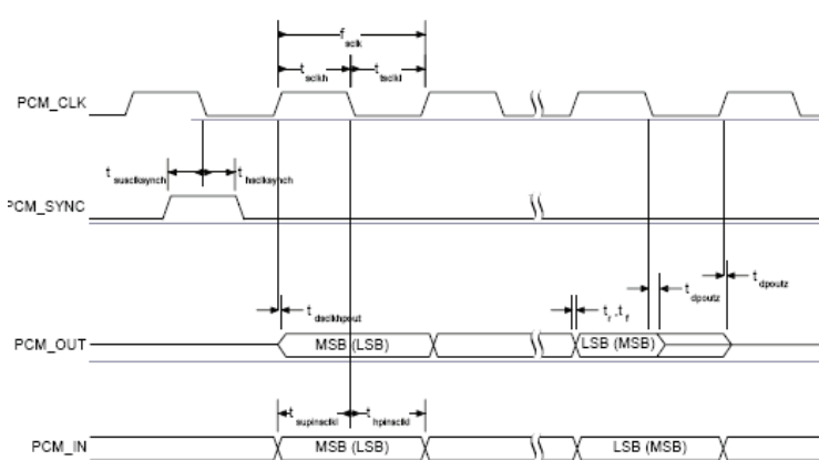
Figure 13. PCM Slave Timing Short Frame Sync
