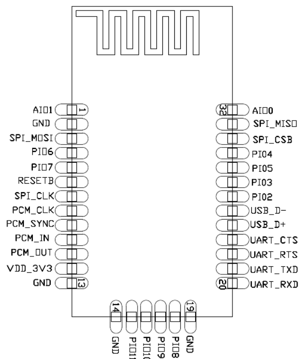
Figure 1. Pinout (Topview)
