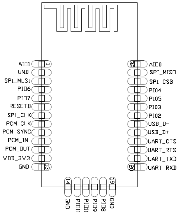
Figure 1. Pinout (Topview)
