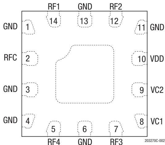
Figure 2. SKY13575-639LF Pinout (Top View)
