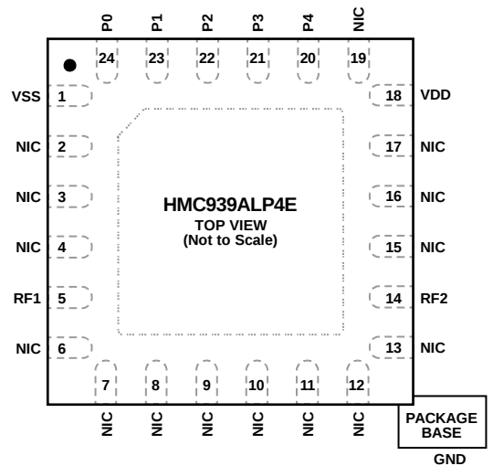
Figure 2. Pin Configuration
