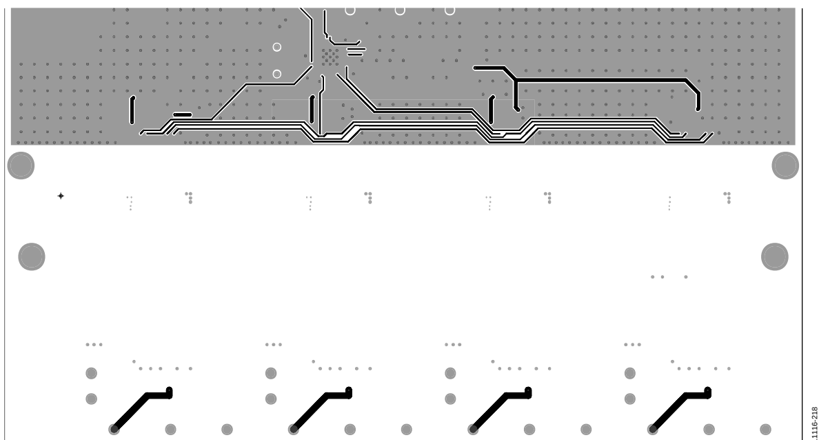
Figure 123. ADE7978, ADE7933, and ADE7923 Circuit Board, Layer 4
