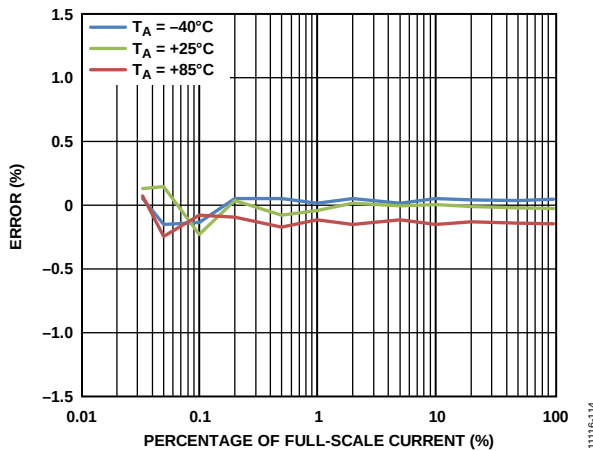
Figure 15. Total Reactive Energy Error as a Percentage of Reading over Temperature, PF = 0
