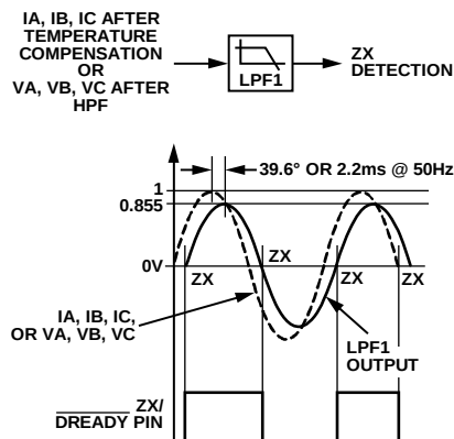
Figure 61. Zero-Crossing Detection on Voltage and Current Channels
