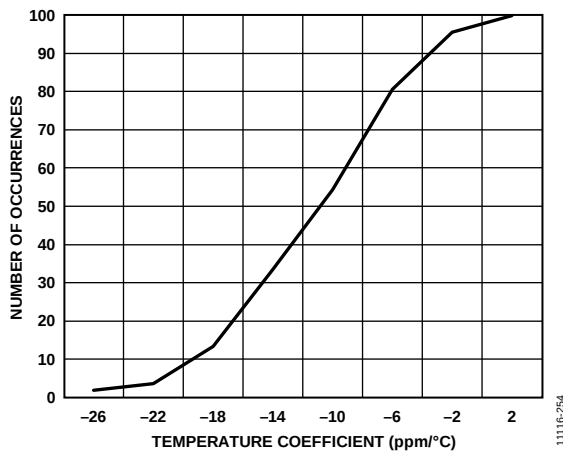
Figure 38. Cumulative Histogram of the ADE7932/ADE7933/ADE7923 Voltage Channel V1 ADC Gain Temperature Coefficient for Temperatures Between -40^{\circ}\text{C} and +25^{\circ}\text{C}
