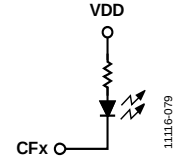
Figure 93. CFx Pin Recommended Connection
