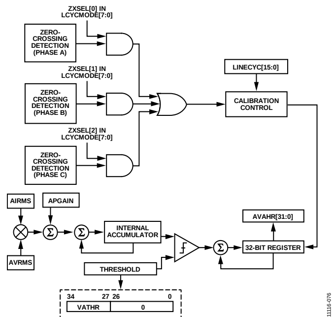
Figure 90. Line Cycle Apparent Energy Accumulation Mode
