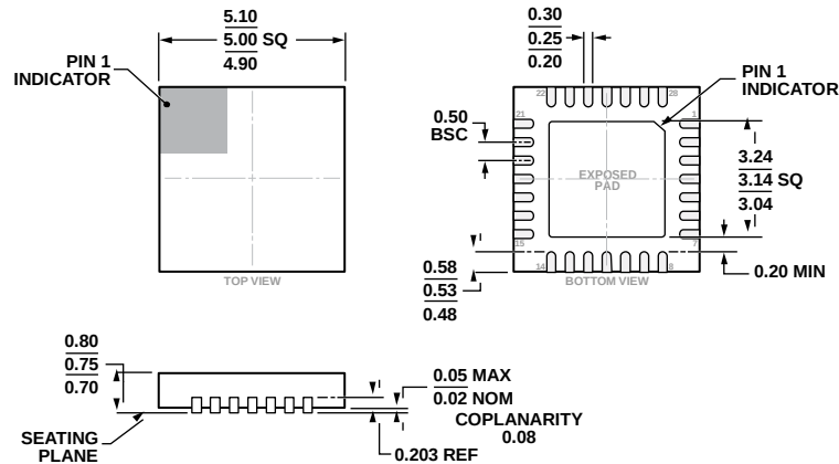
Figure 138. 28-Lead Lead Frame Chip Scale Package [LFCSP] 5 mm × 5 mm Body and 0.75 mm Package Height (CP-28-10)
