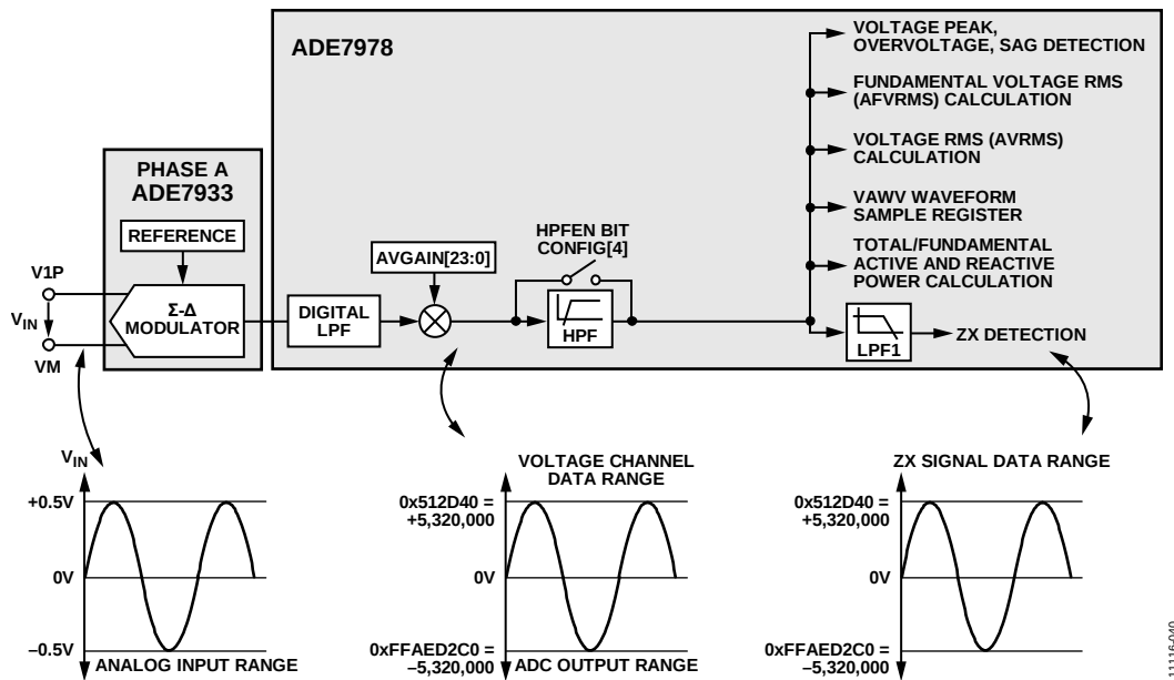
Figure 54. Phase A to Neutral Voltage Channel Datapath
