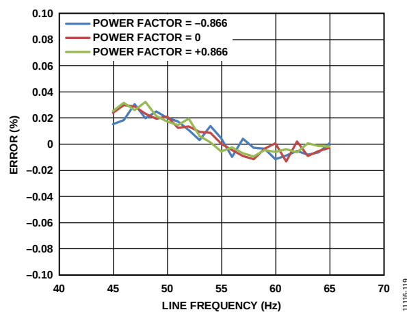
Figure 27. Total Reactive Energy Error as a Percentage of Reading over Frequency, PF = -0.866, 0, and +0.866
