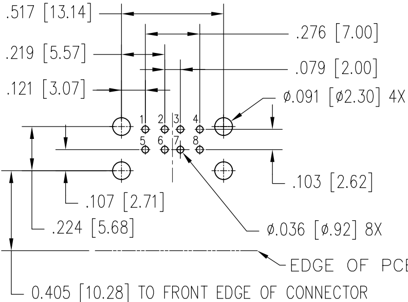
RECOMMENDED P.C.B HOLE LAYOUT TOP VIEW (TOLERANCE: ±.004 [±0.10])
