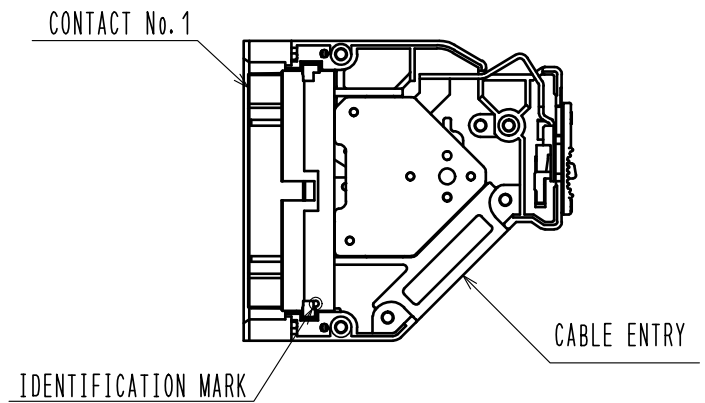
FIG.1 ASSEMBLY DRAWING (1:2)
