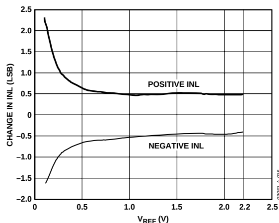
Figure 16. Change in INL vs. V_{REF} for the AD7450A for V_{DD} = 3\text{ V}
