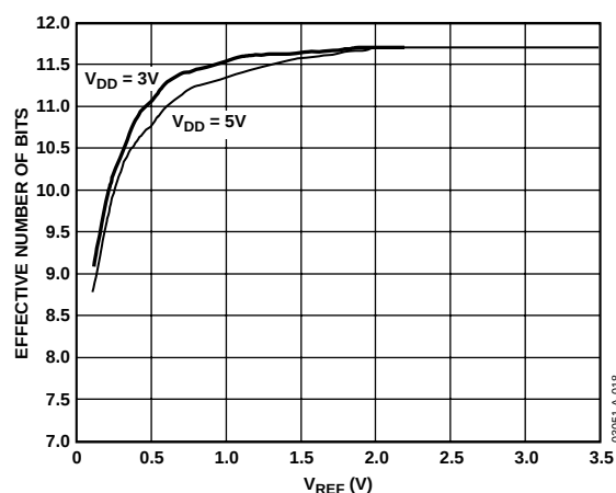
Figure 18. Change in ENOB vs. Reference Voltage for V_{DD} = 5\text{ V} and 3\text{ V} for the AD7450A
