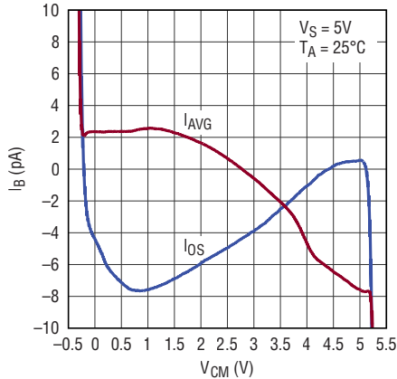
Input Offset and Average Current vs Input Common Mode Voltage
