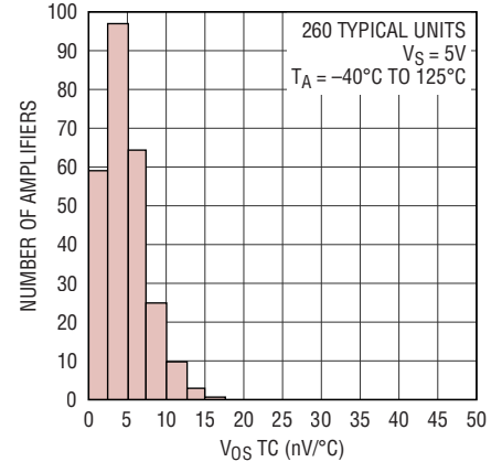
Input Offset Voltage Drift Distribution (H-Grade)
