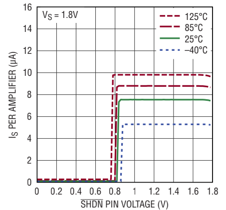
Supply Current vs \overline{SHDN} Pin Voltage
