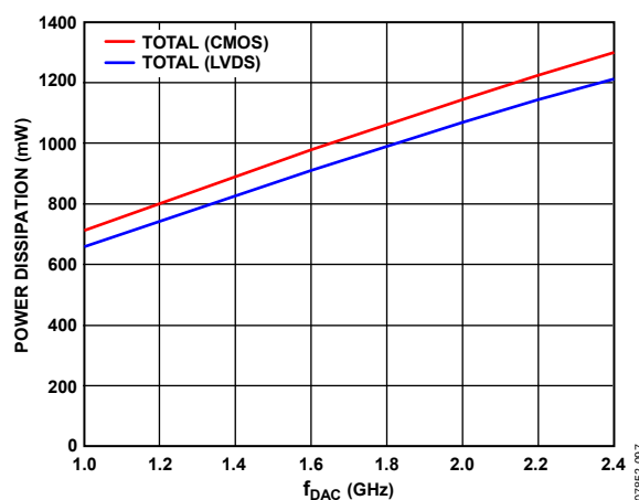
Figure 61. Total Power Dissipation vs. f_{DAC} , 16x Interpolation, One Channel Enabled, f_{OUT} = 70 MHz, Full-Scale Current = 20 mA
