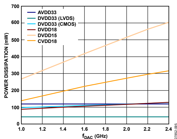
Figure 58. Power Dissipation by Supply vs. f_{DAC} , 16x Interpolation, One Channel Enabled, f_{OUT} = 70 MHz, Full-Scale Current = 20 mA
