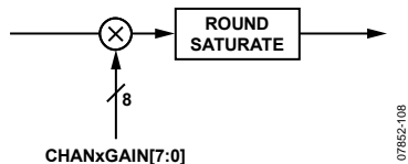
Figure 85. Individual Channel Gain Control
