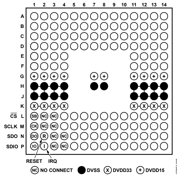
Figure 6. Digital Supply and SPI Pins (Top View)
