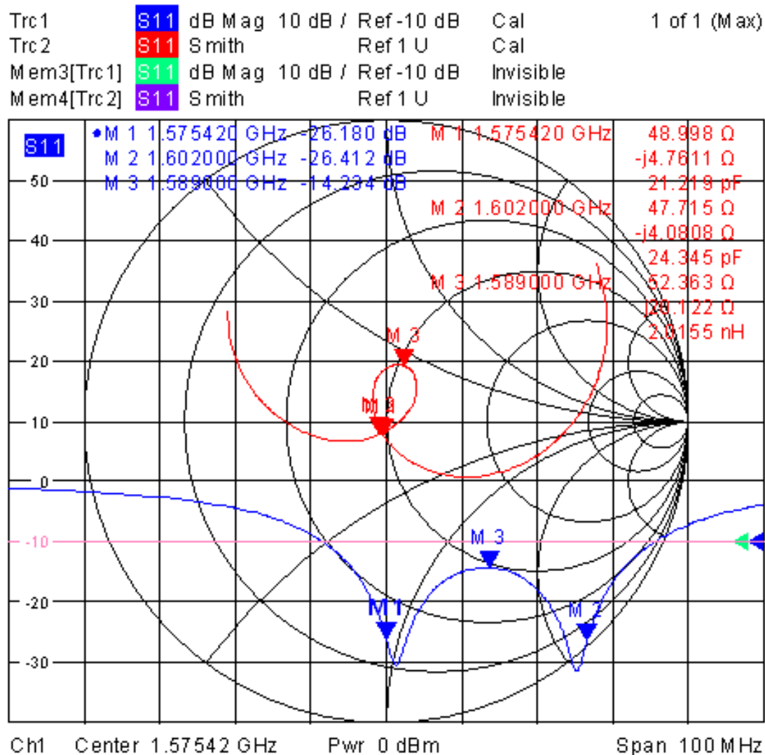
Fig. 3 Return loss
