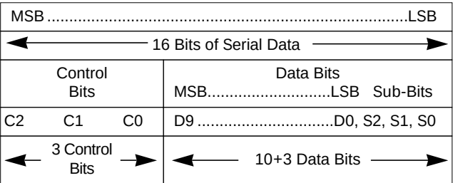
Figure 4. Serial-Data Format
