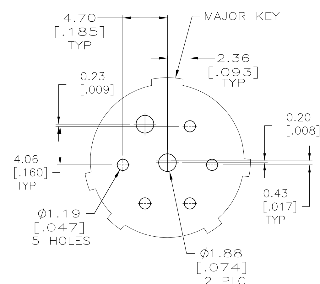
RECOMMENDED BOARD LAYOUT FOR 788194-6 ONLY SCALE 4:1
