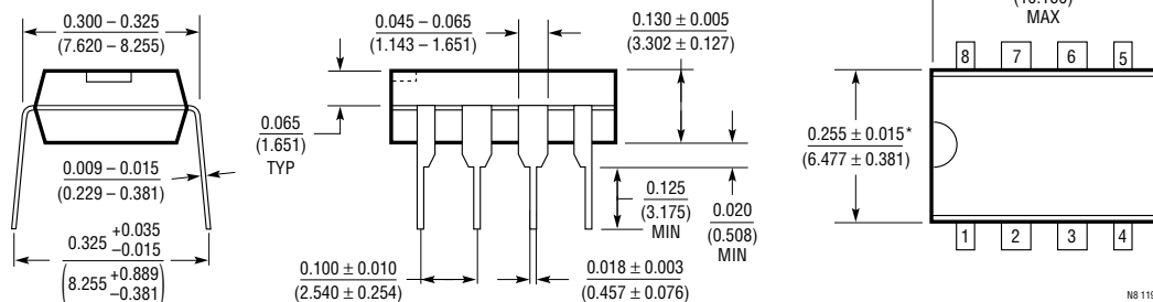
N8 Package 8-Lead PDIP (Narrow 0.300) (LTC DWG # 05-08-1510)
