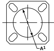
BACK PANEL MOUNTING
