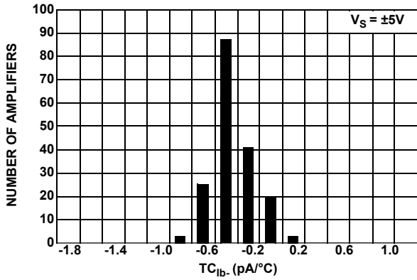
FIGURE 15. TC ib- vs NUMBER OF AMPLIFIERS, V S = ±5V
