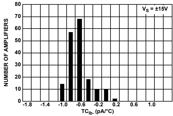
FIGURE 16. TC ib- vs NUMBER OF AMPLIFIERS, V S = ±15V
