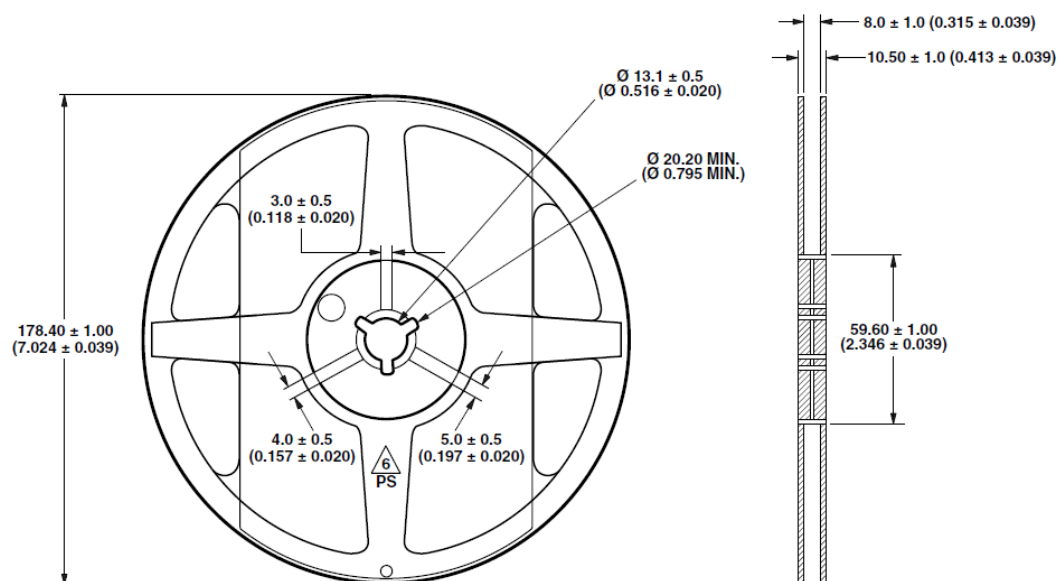
Figure 13: Reel Dimensions
