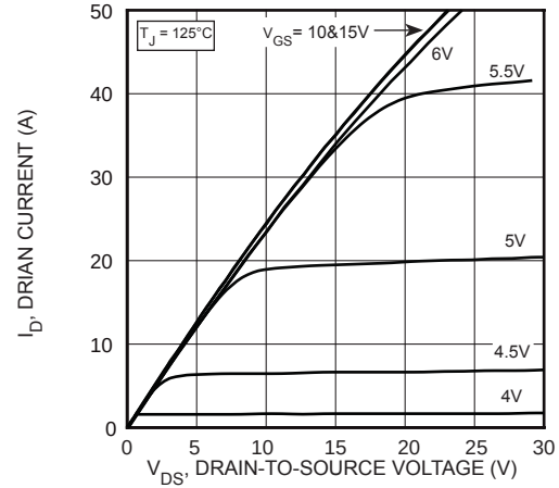
Figure 2, Output Characteristics
