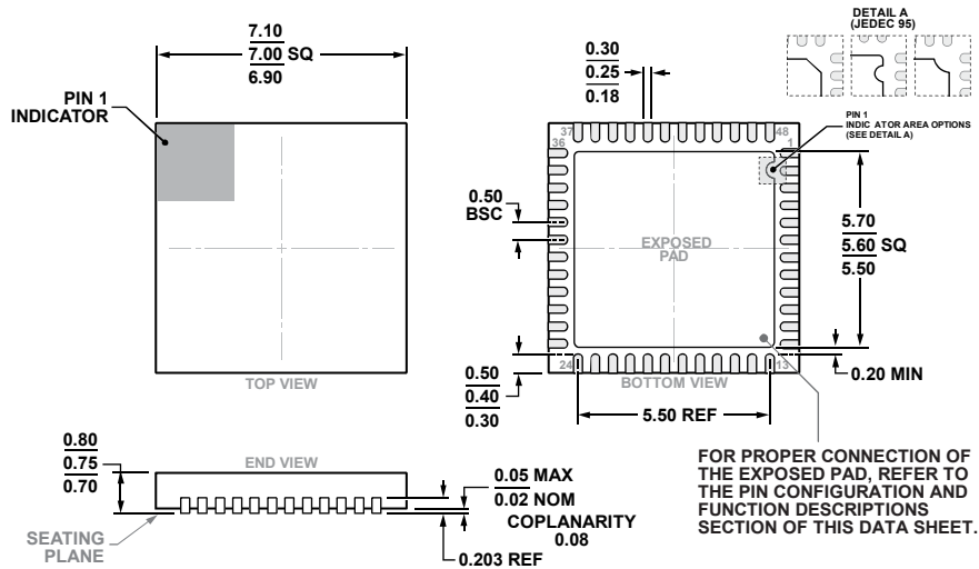
Figure 77. 48-Lead Lead Frame Chip Scale Package [LFCSP] 7 mm × 7 mm Body and 0.75 mm Package Height (CP-48-13)
