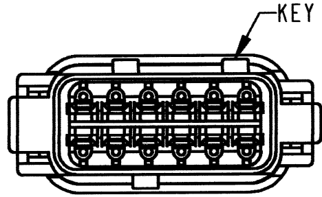
DTM06-12SB-E007 KEY -B- COLOR: BLACK
