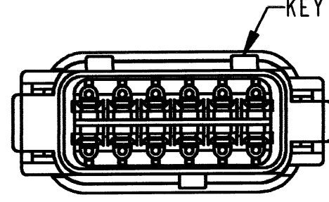
DTM06-12SD-E007 KEY -D- COLOR: BROWN
