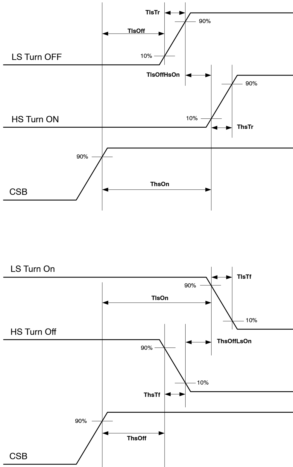
Figure 4. Detailed Driver Timing
