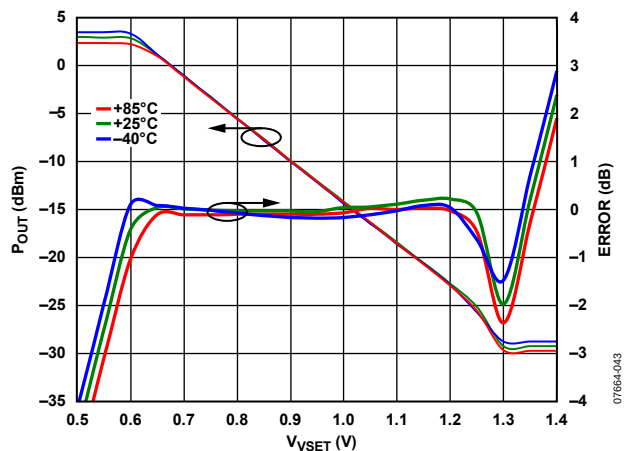
Figure 43. P_{OUT} vs. V_{VSET} Transfer Function in AGC Mode (1 V p-p Differential Baseband Input Voltage on I and Q)
