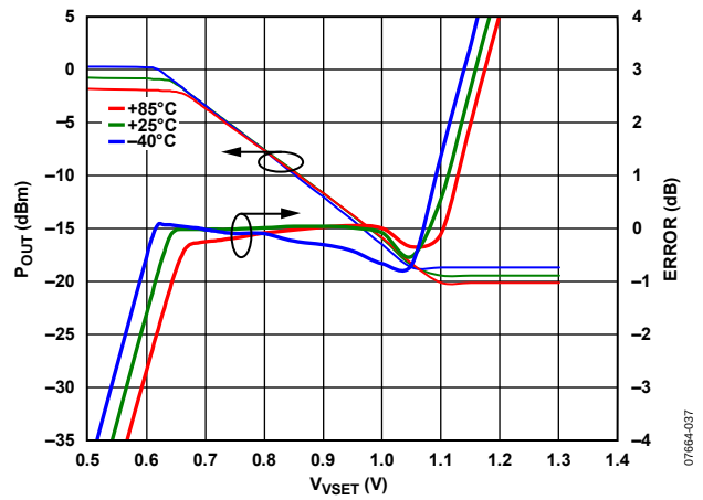
Figure 37. P_{\text{OUT}} and Error vs. V_{\text{VSET}} at 1900 MHz
