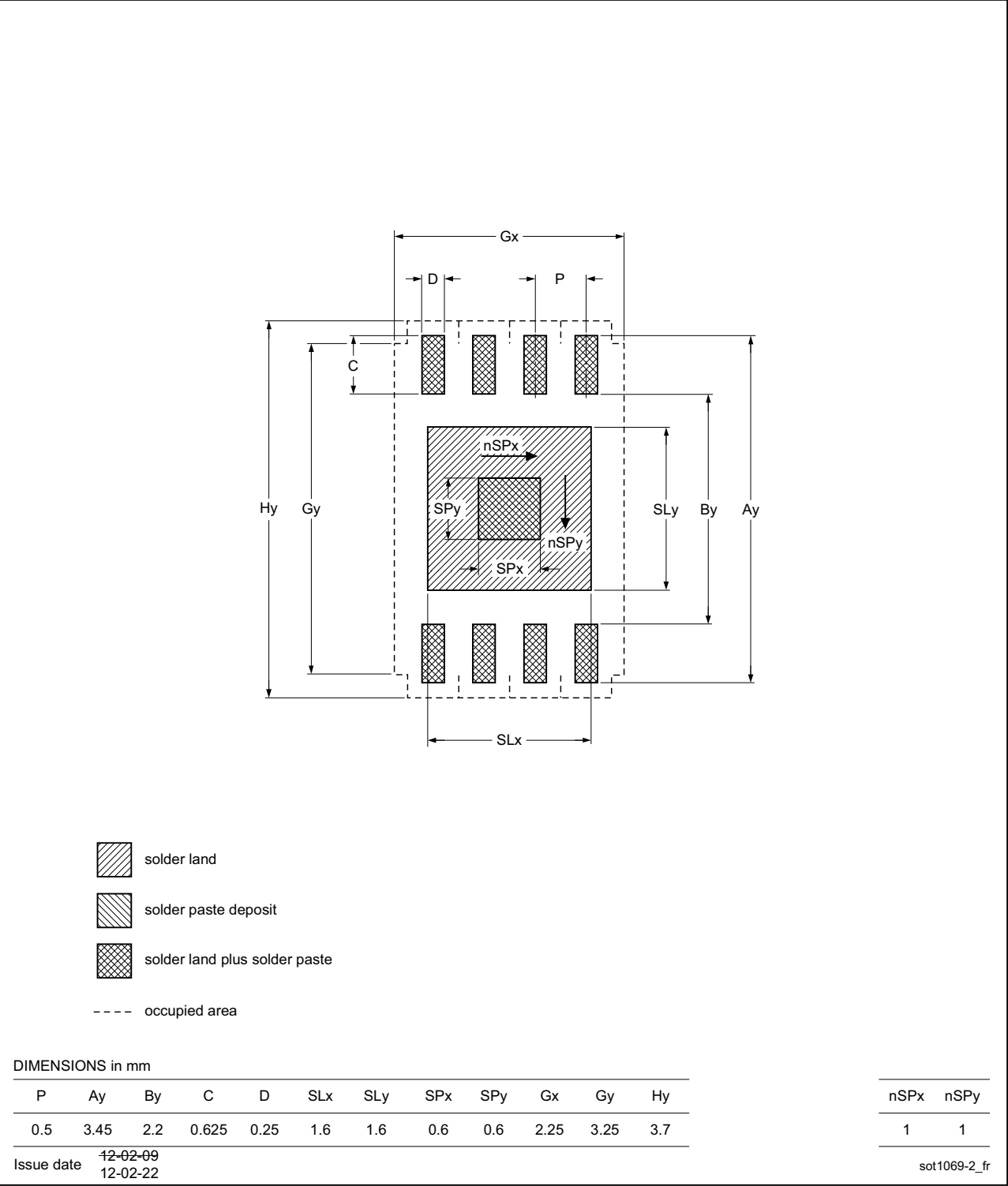
Fig 30. PCB footprint for SOT1069-2 (HWSON8); reflow soldering
