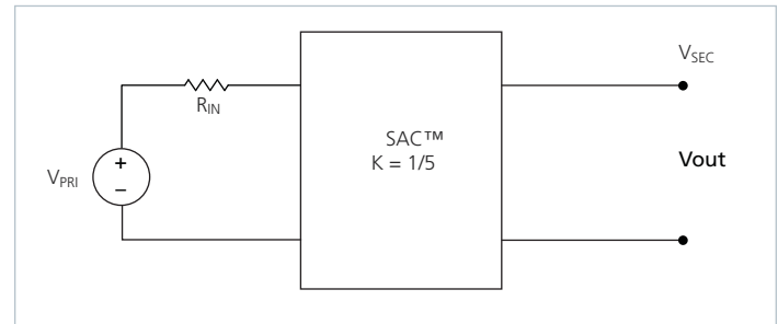
Figure 17 — K = 1/5 Sine Amplitude Converter with series input resistor
