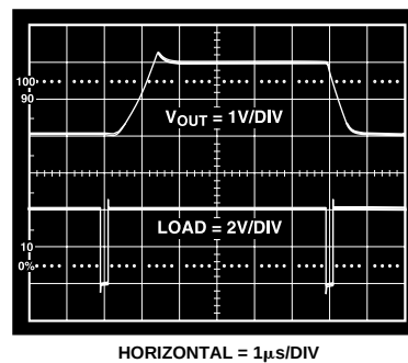
Figure 6. Detail Settling Time
