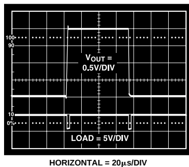
Figure 9. Large Signal Settling Time
