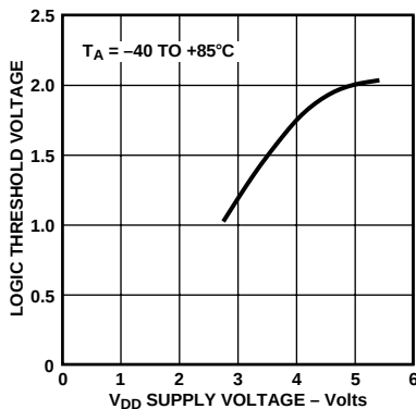
Figure 5. Logic Input Threshold Voltage vs. V_{DD}
