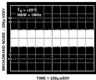
Figure 7. Broadband Noise
