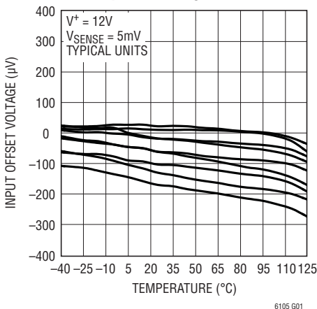
Input Offset Voltage vs Temperature, V_S^+ = 12\text{V}
